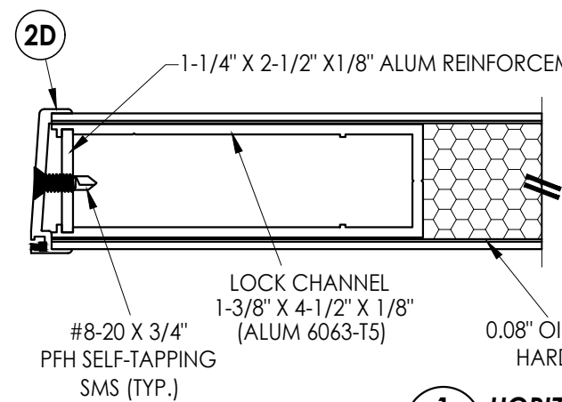
1 2 HORIZONTAL CROSS SECTION
