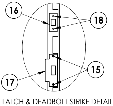
LATCH & DEADBOLT STRIKE DETAIL
