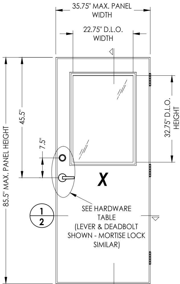
2 2 40 VENTED DOOR PANEL
