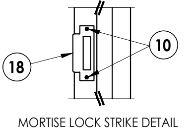
MORTISE LOCK STRIKE DETAIL
